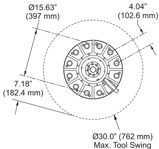
12-Station VDI Turret Option
