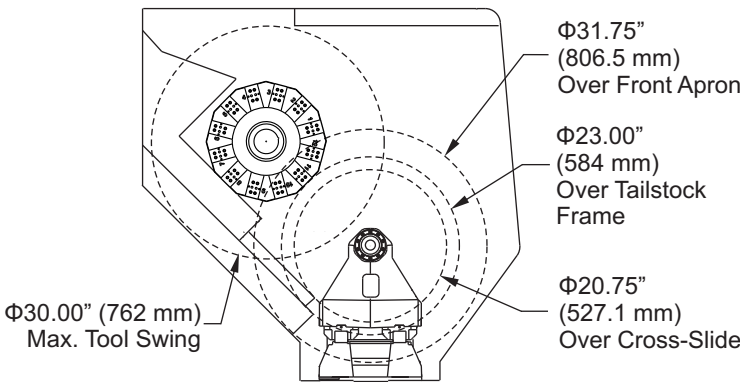
ST-20/25 Tool Swing Envelope Turret at Home Position 12-Station BOT Turret Standard 12-Station VDI Turret Standard in HAE only
